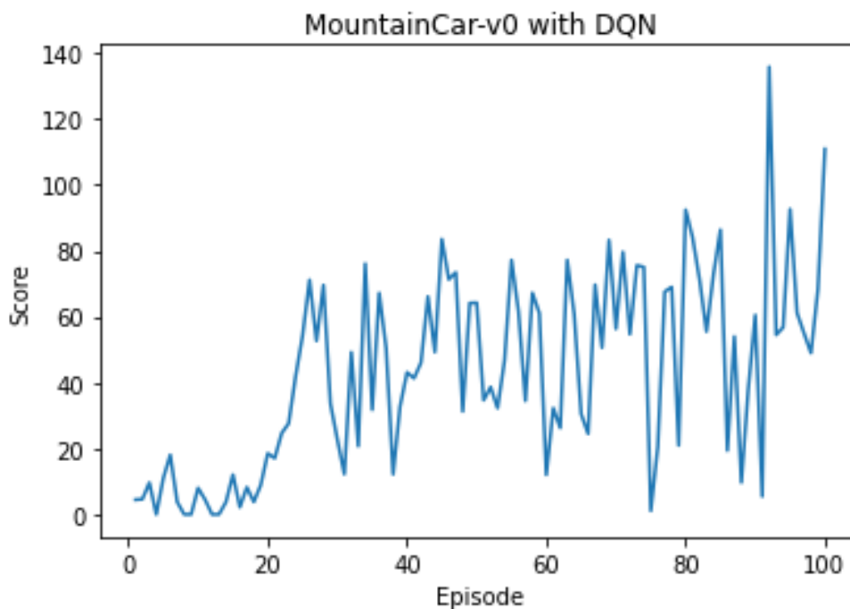
Figure 5.9: total reward per episode using pytorch
