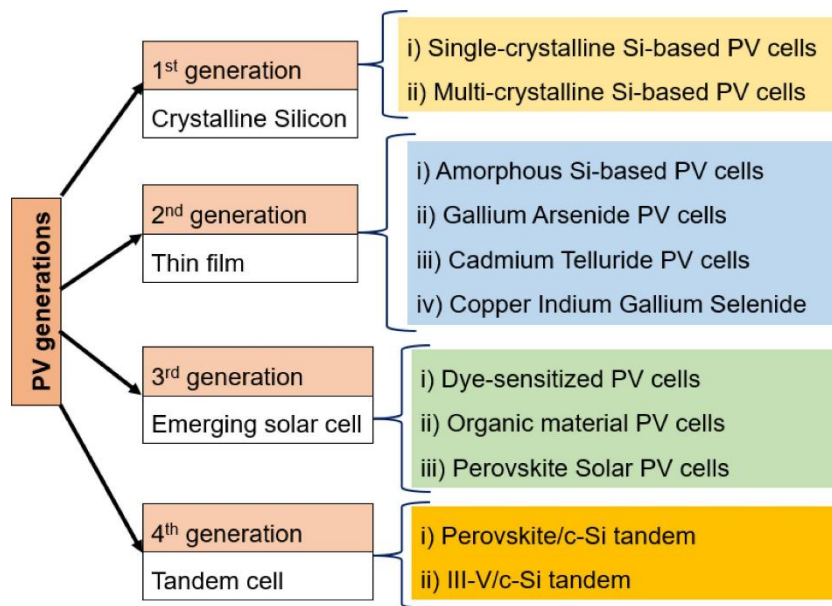
Figure 1.1 PV generations [2]
