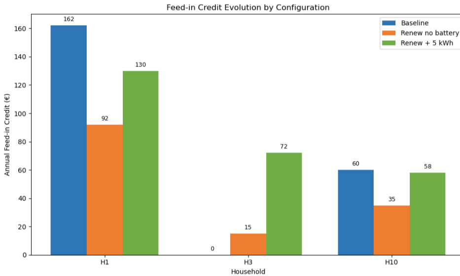
Figure 4.19 Feed-in credit evolution by configuration
