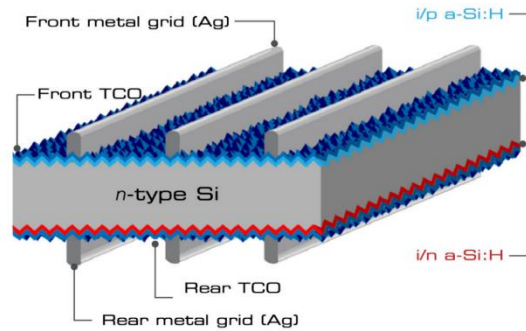
Figure 1.9 Structure of Monocrystalline silicon cell [8]
