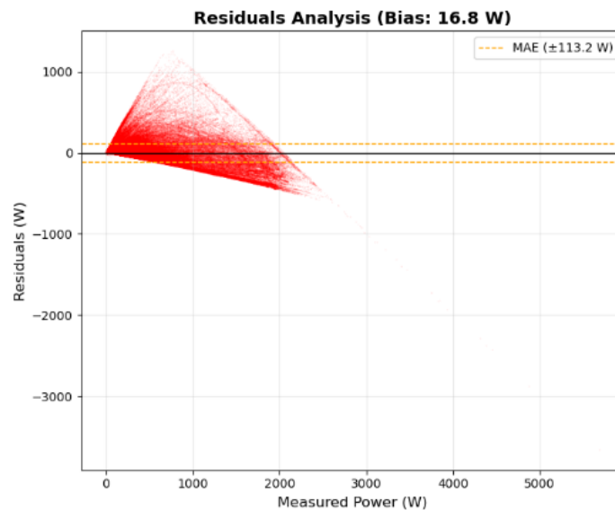
Figure 4.14 Residual analysis
