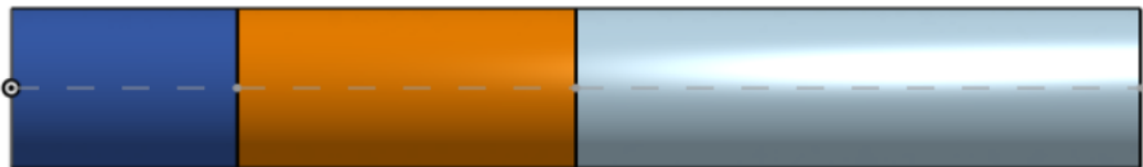
Figure 8.3: Geometric representation of the linear vessel using Onshape software. The blue section refers to the vessel before the scaffold, with a length of 10 cm. The orange section represents the scaffold, with a length of 15 cm, while the silver section corresponds to the vessel after the scaffold, with a length of 25 cm.
