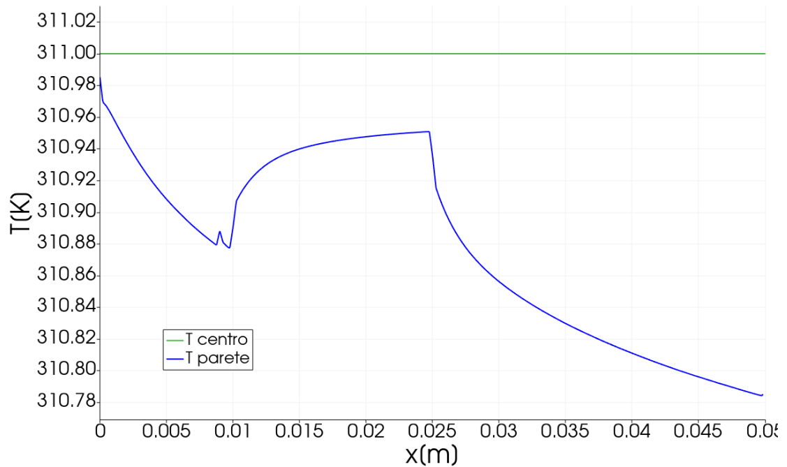
Figure 10.3: Temperature profile along the axis of the linear vessel with a diameter of 2.5 mm. The central temperature remains constant along the length of the vessel, while the wall temperature shows a progressive decrease, with a rise in correspondence with the scaffold. This behavior is attributable to the scaffold's lower heat exchange capacity compared to the natural vascular wall, which leads to reduced heat dissipation in this region.
