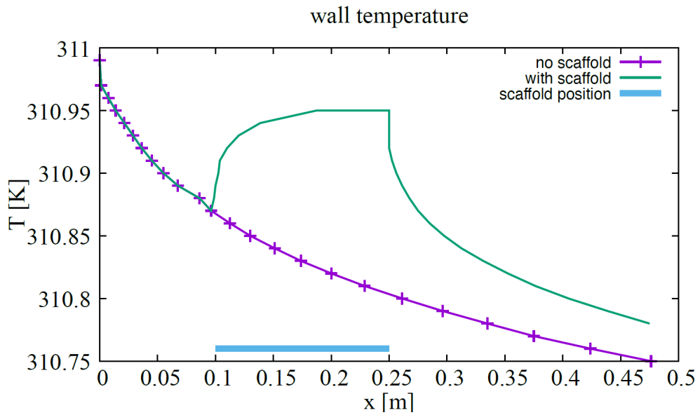
Figure 10.36: Comparison of the wall temperature profiles along the longitudinal axis for two linear vessels (diameter = 3.5 mm): one including the scaffold (green curve) and one without it (purple curve). The position of the scaffold is indicated by the blue region. The scaffold introduces a localized region of slightly increased temperature due to altered heat transfer dynamics. However, as clearly depicted, this increase remains well below 0.2 degrees (applicable to both Kelvin and Celsius), confirming that the thermal effect of the scaffold is minimal and clinically negligible.
