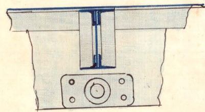
Plan of Bracket & Davit Socket on longer Plate Scale 1" = one foot
