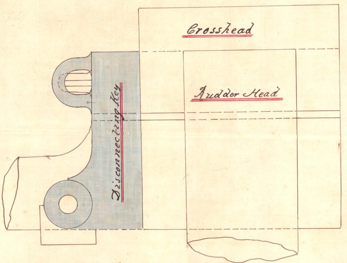
Elevation of Disconnecting Gear Half Size
