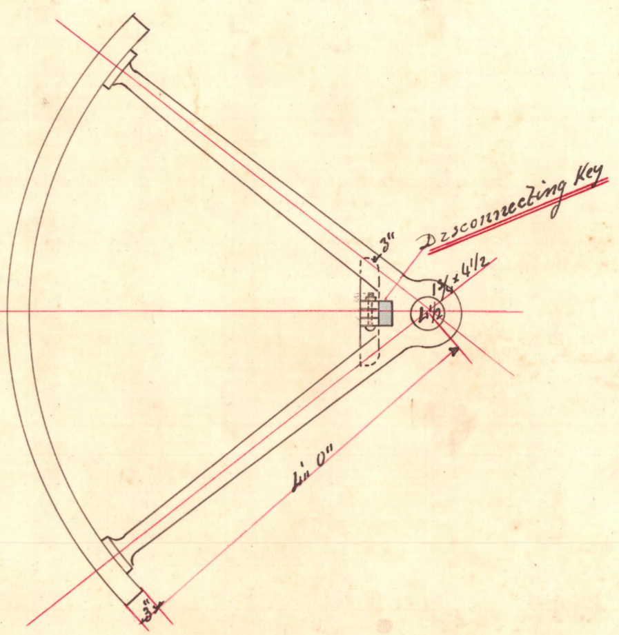
Plan of Quadrant
