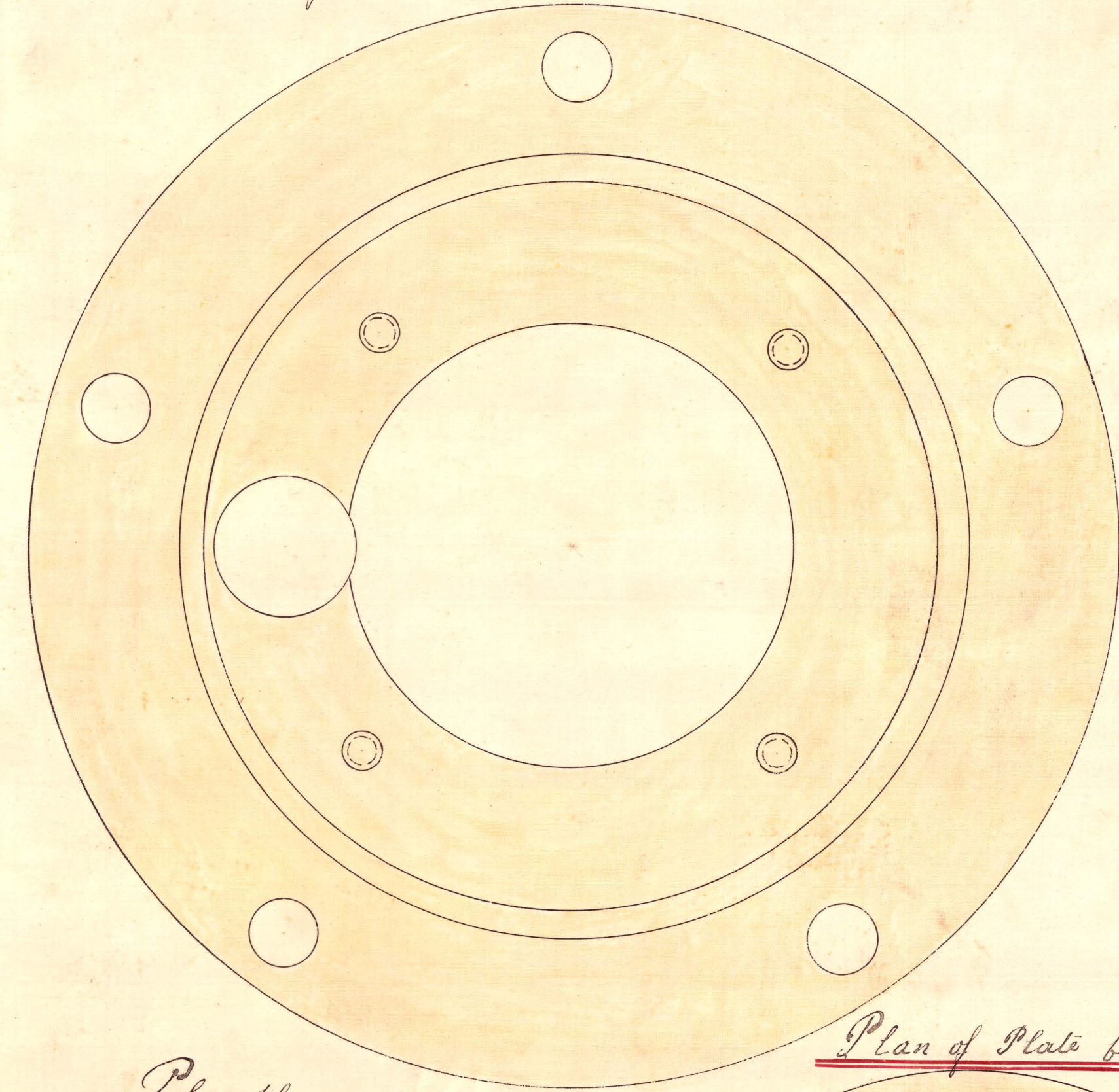
Plan of Deck plate a a a
