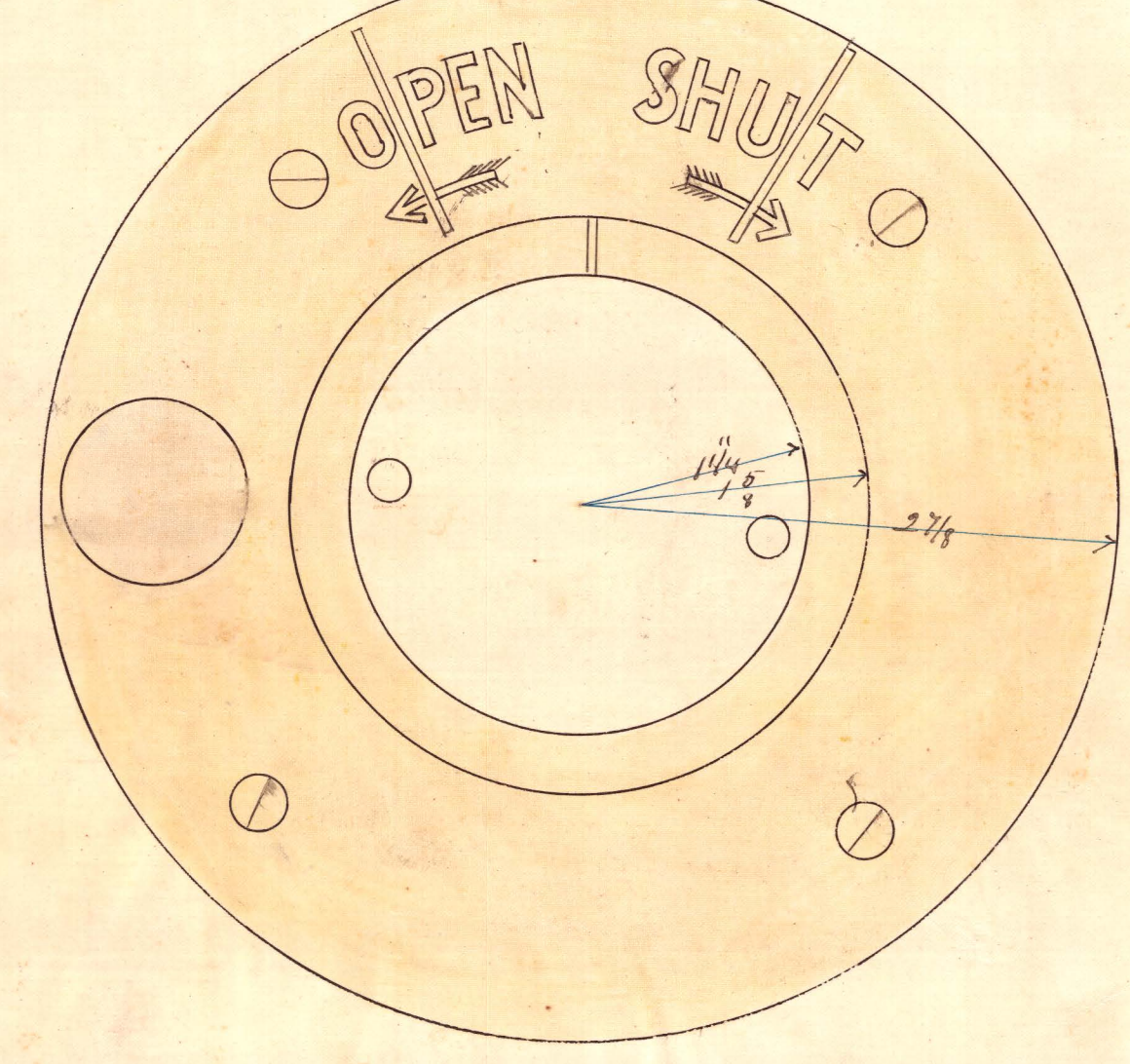
Elevation of plate b
